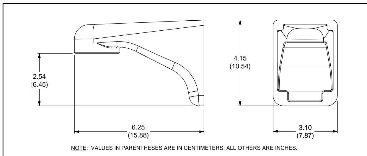
Figure 2. SWM Dimension Drawing
